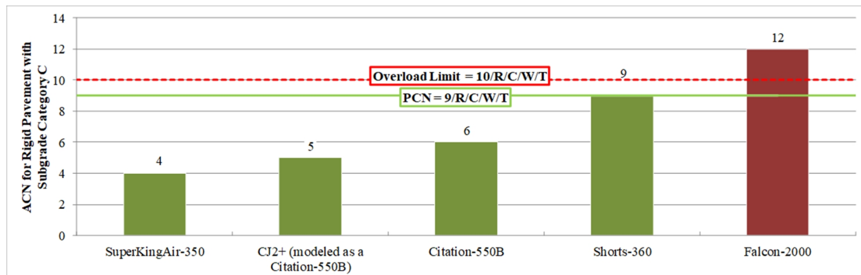
Figure 1. ACN–PCN comparison for Runway 11-29.
