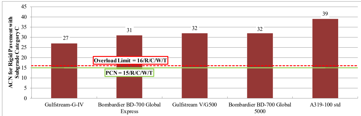
Figure 1. ACN–PCN comparison for Runway 7/25.
