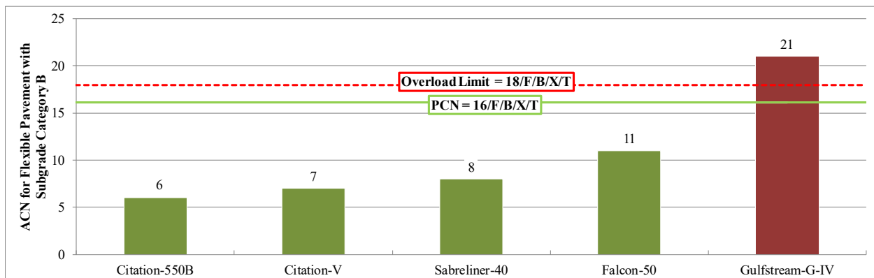
Figure 1. ACN–PCN comparison for Runway 13-31.
