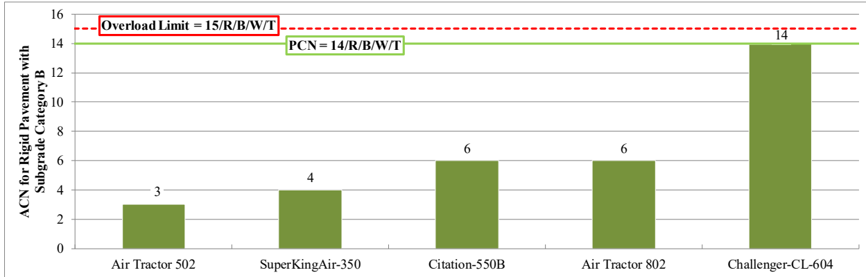
Figure 1. ACN–PCN comparison for Runway 8-26.
