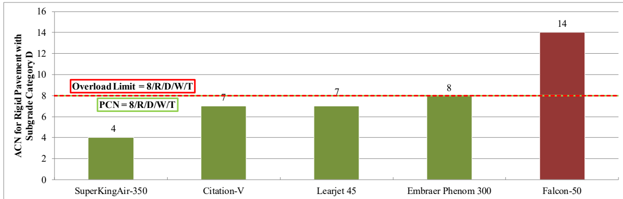
Figure 1. ACN–PCN comparison for Runway 16/34.
