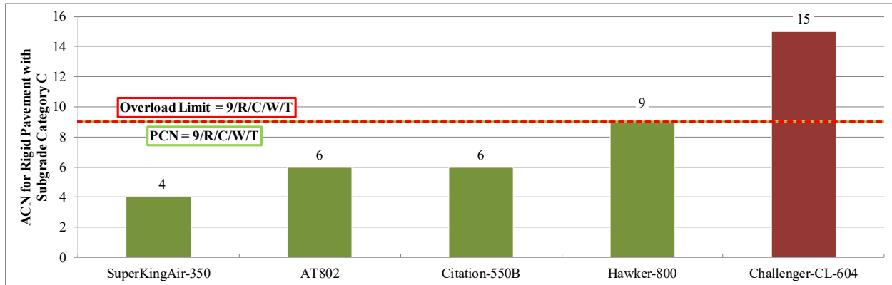
Figure 1. ACN–PCN comparison for Runway 5/23.
