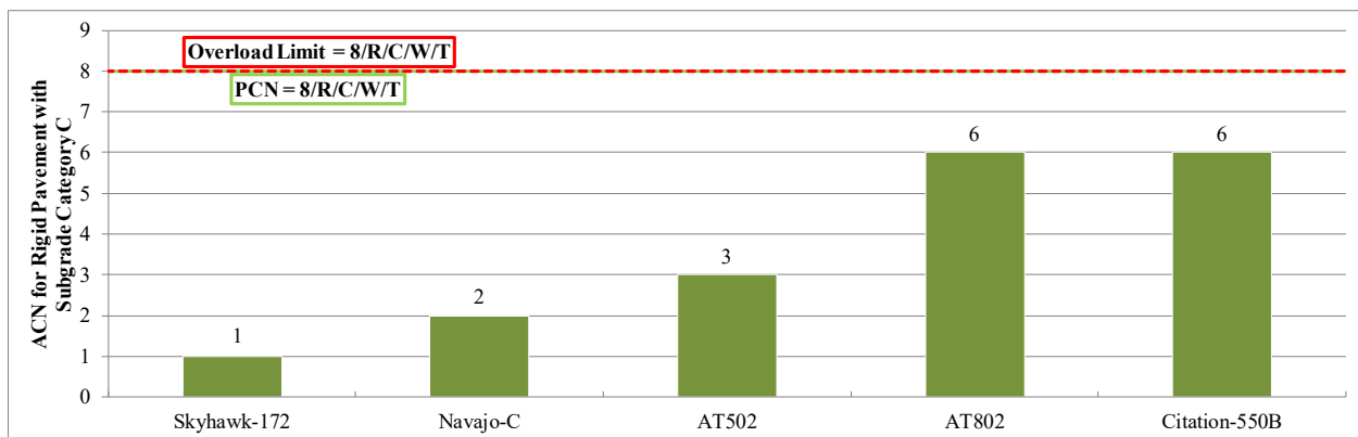
Figure 2. ACN–PCN comparison for Runway 17/35.
