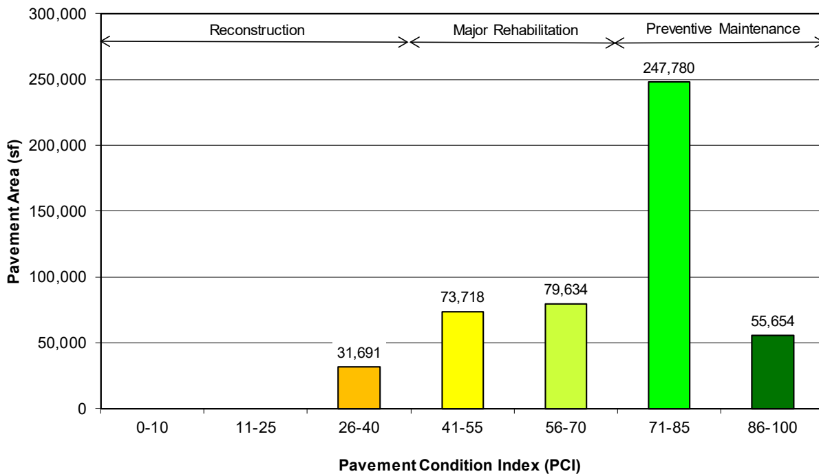
Figure 6. Pavement area by PCI range at Decorah Municipal Airport.
