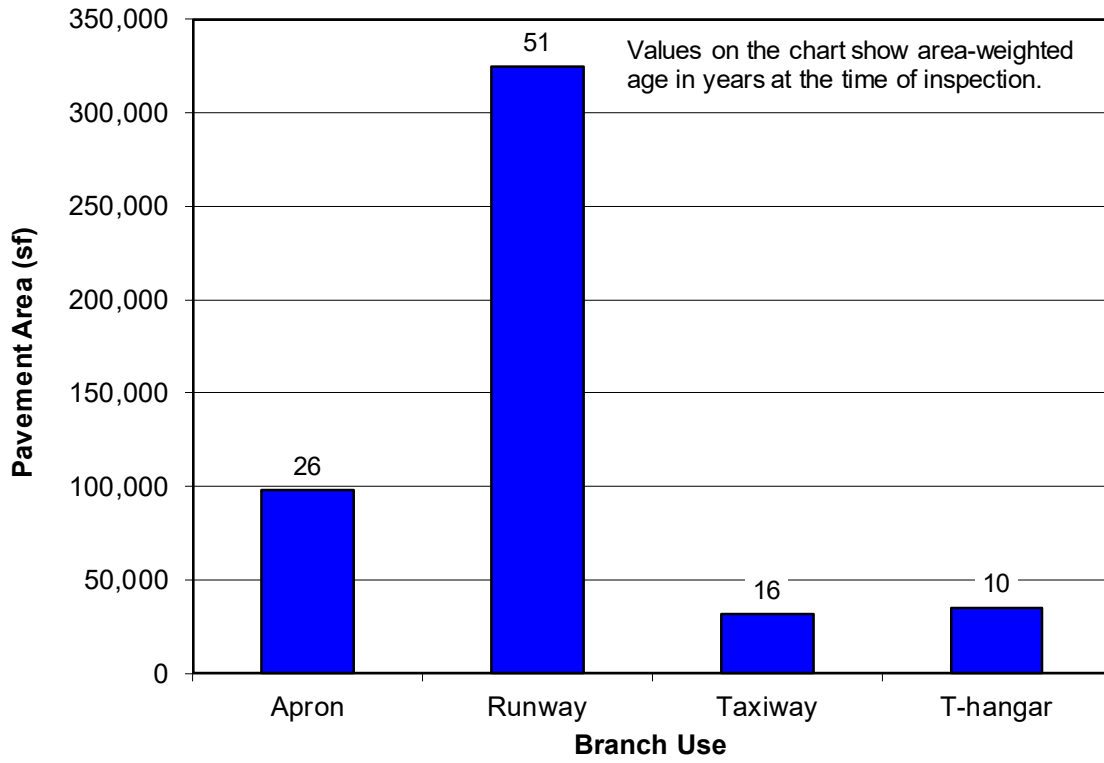
Figure 2. Pavement area by branch use at Decorah Municipal Airport.
