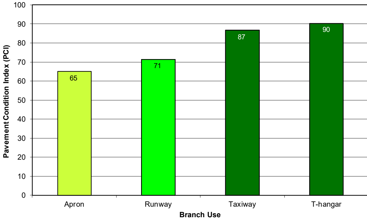
Figure 7. Area-weighted PCI by branch use at Decorah Municipal Airport. (Values on chart are area-weighted)
