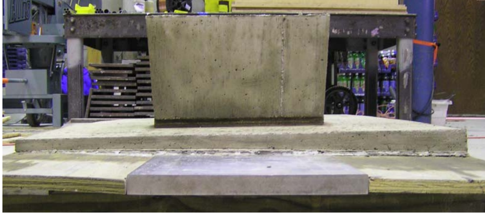
Figure 3.5. Haunch cross-section after form removal.
