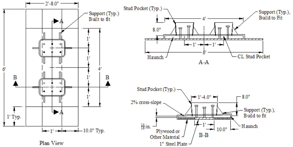
Figure 3.1. Shear Stud/Grout Flow Mock-Up Dimensions.
