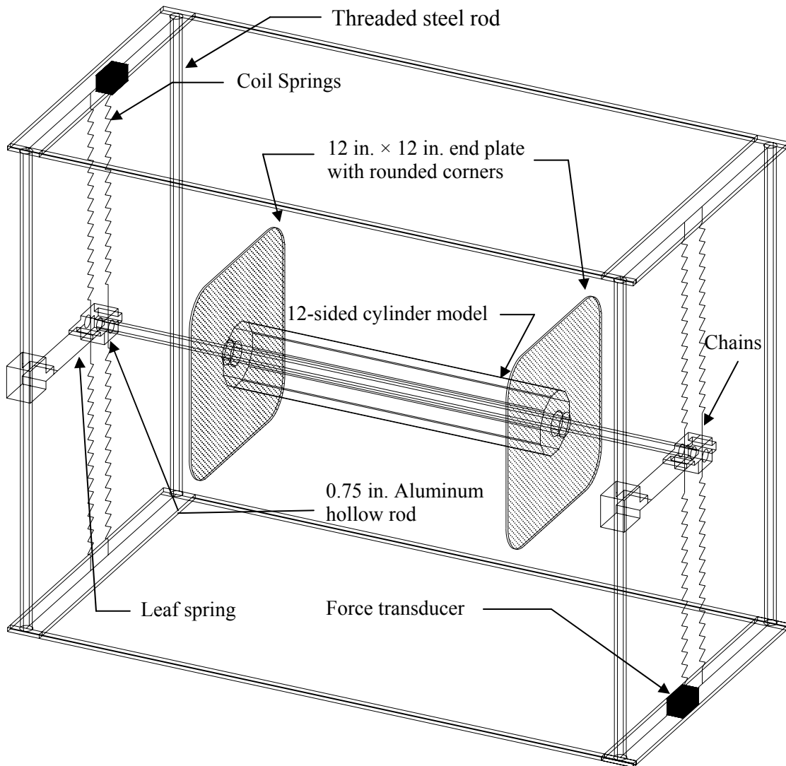
Figure 4-7. Schematic diagram of the general system for the dynamic test
