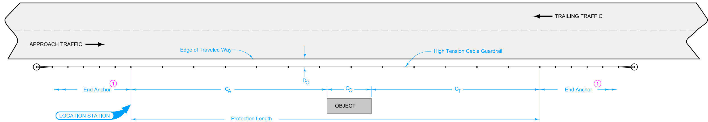
ROADSIDE OBJECT, TWO-WAY PROTECTION
