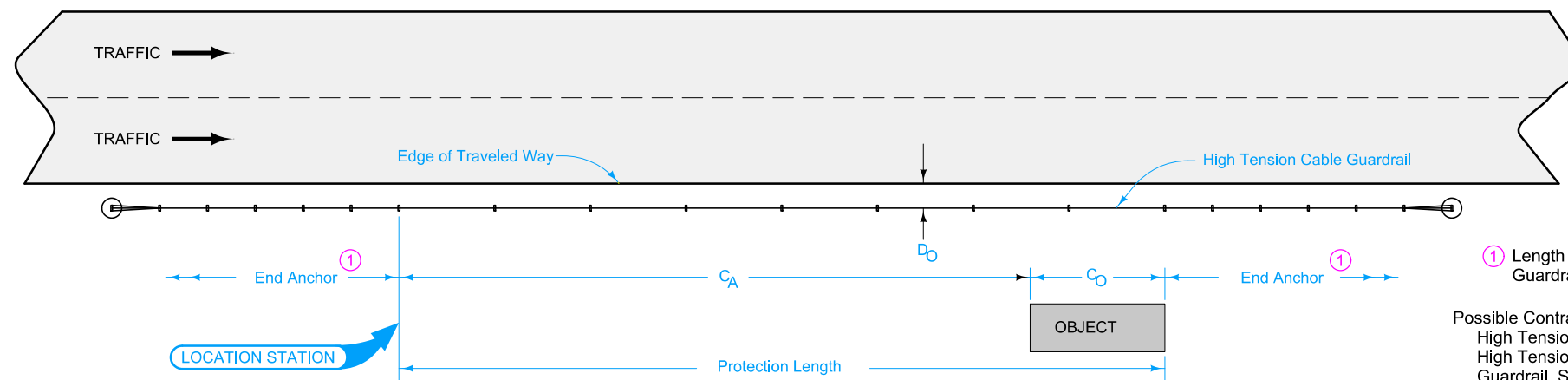
ROADSIDE OBJECT, ONE-WAY PROTECTION
