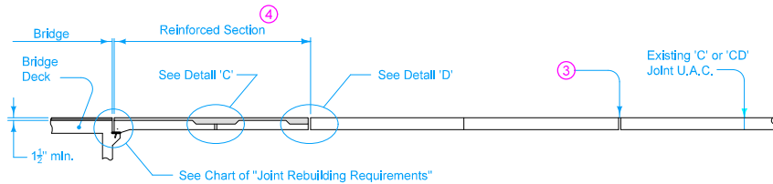
TYPICAL SECTION THRU CENTERLINE
