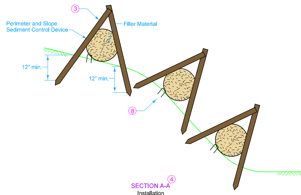
SLOPE PROTECTION 4
