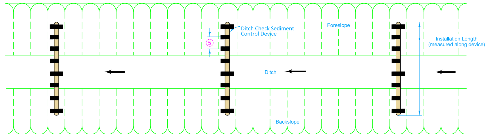
DITCH PROTECTION 6
