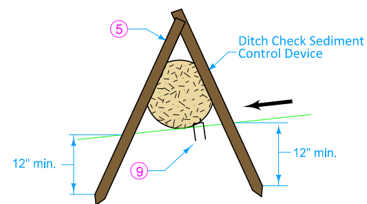
INSTALLATION IN DITCH
