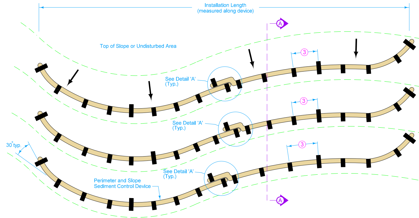
SLOPE PROTECTION 4
