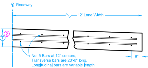
SECTION A-A Half Section
