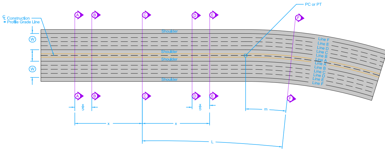
TRANSITION DETAILS - TANGENT TO CURVE
