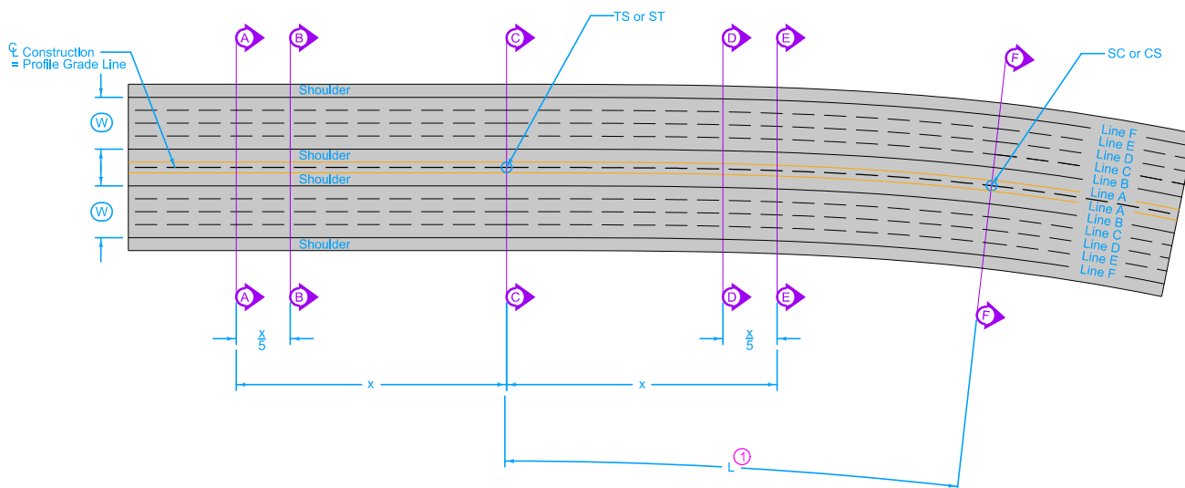
TRANSITION DETAILS - SPIRAL CURVE
