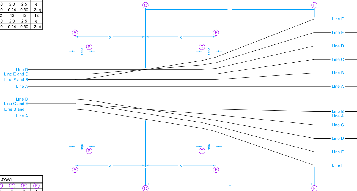
DIAGRAMMATIC PROFILES OF THE PAVEMENT EDGE LINES
