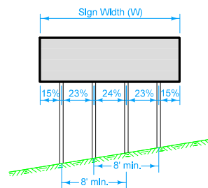
Four Post Erection POST POSITION DETAIL
