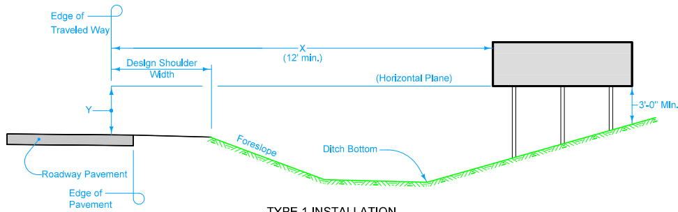
TYPE 1 INSTALLATION (OFFSET)
