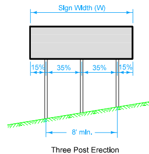
Three Post Erection
