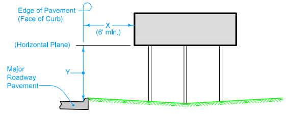
TYPE 2 INSTALLATION (CURBED SECTION)
