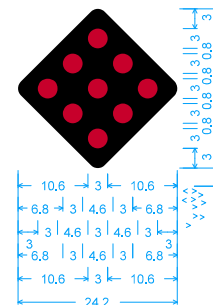
DEAD END WITH CUL-DE-SAC
