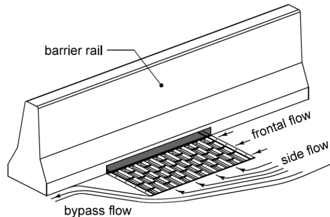
Figure 1: Grate intake flow definitions.
