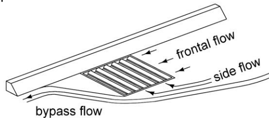
Figure 3: Intake bridge end drain flow definitions.
