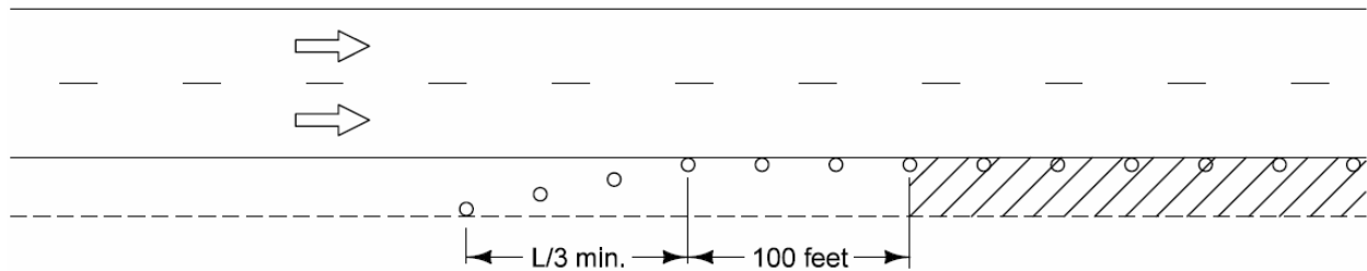
Figure 3: Shoulder taper.
