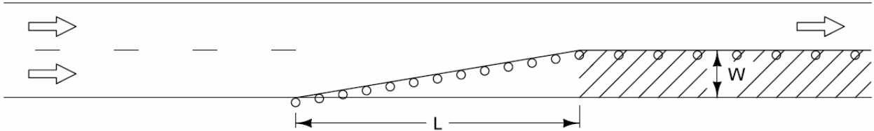
Figure 1: Merging taper.
