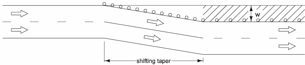
Figure 2: Shifting taper.
